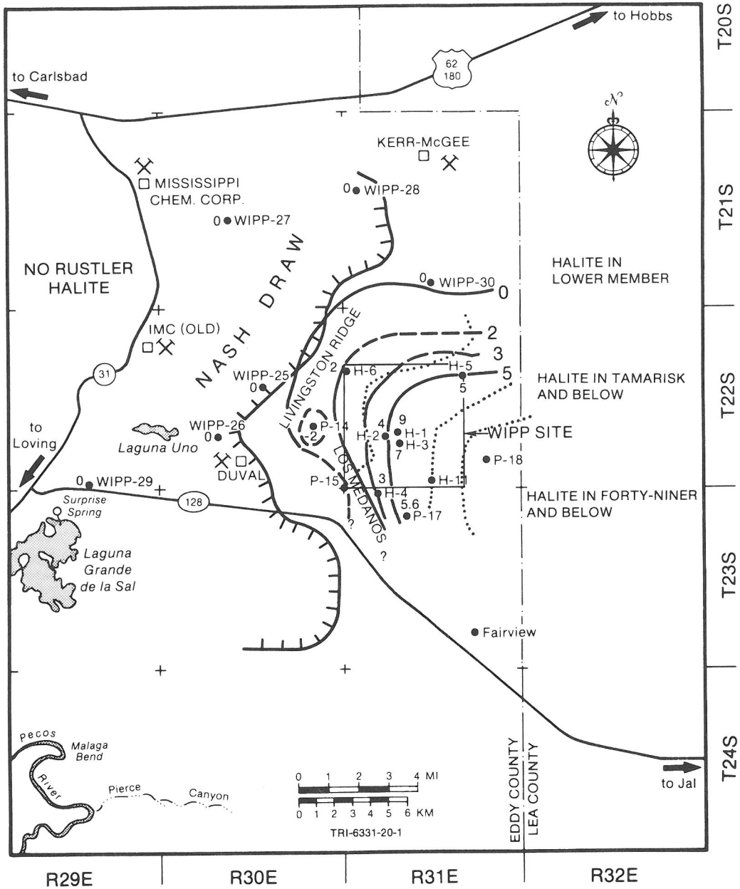
FIG. 8. Contour map of oxygen-isotope deviation in confined groundwaters at the Rustler/Salado contact, relative to \delta^{18}\text{O} = -7 . Dotted lines are boundaries of SNYDER (1985) delineating the occurrences of halite in various members of the Rustler.
