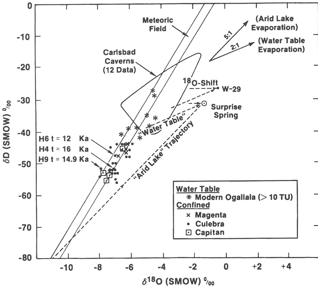
FIG. 6. Stable-isotope compositions of confined groundwaters from the Rustler Formation and Capitan Limestone. The isotopic compositions of demonstrably modern Ogallala groundwaters containing significant ( >10 TU) tritium are shown for comparison.
