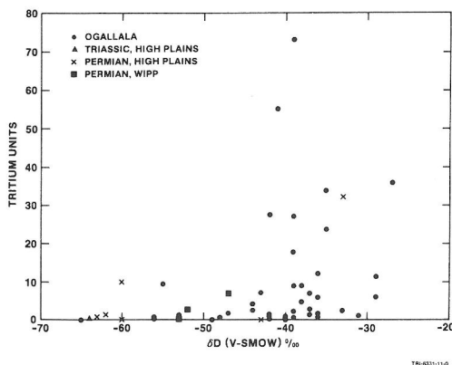
FIG. 4. Tritium and deuterium concentrations in groundwaters from the Southern High Plains, Texas, and the Delaware Basin, southeastern New Mexico. High Plains data are from NATIV and SMITH (1987).
