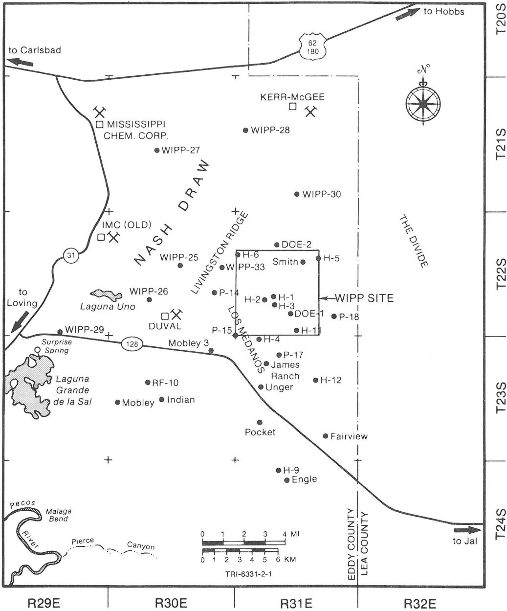
FIG. 2. Map of northern Delaware Basin, southeastern New Mexico. Detailed map of the area enclosed by hachures in Fig. 1 showing sampling localities, mostly borcholes. Modified from MERCER (1983).
