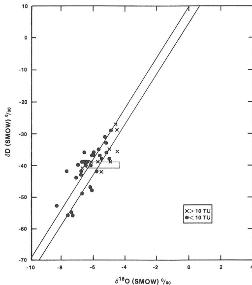
FIG. 5. Stable-isotope compositions of groundwaters from the Southern High Plains, Texas. Data are from NATIV and SMITH (1987). The \delta D range of Ogallala groundwaters (rectangle) from southeastern New Mexico analyzed by YAPP (unpublished) is shown for comparison.
