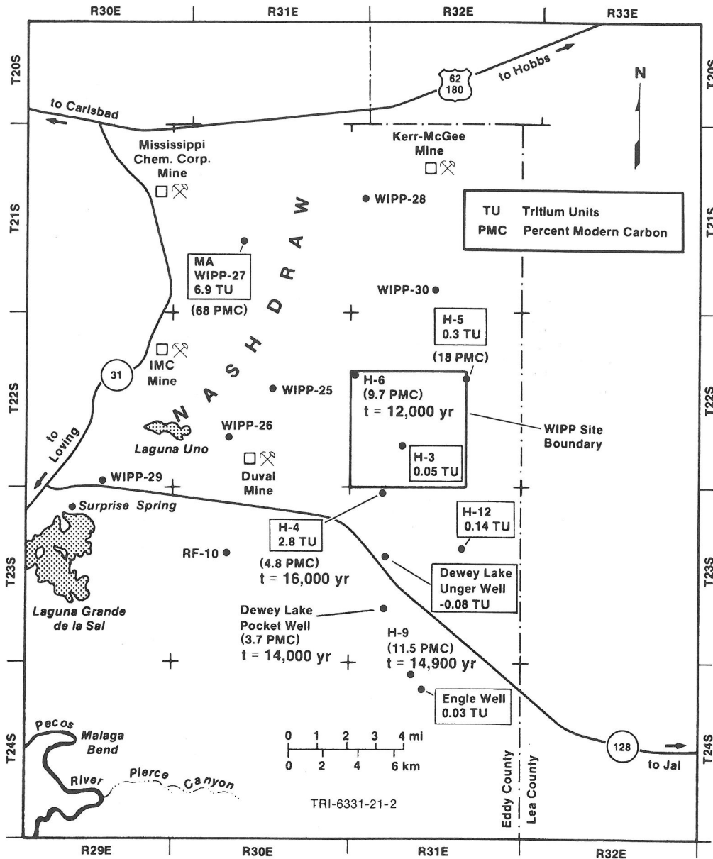
FIG. 9. Tritium and radiocarbon in Rustler and Dewey Lake groundwaters. Unless otherwise specified as Dewey Lake or Magenta (MA), measurements apply to water from the Culebra member of the Rustler Formation. Tritium Units (TU, 1 part tritium in 10^{18} total hydrogen) enclosed in rectangles. The PMC values at H-5 and WIPP-27 are probably contaminated.
