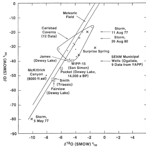
FIG. 3. Stable-isotope compositions of near-surface waters and shallow groundwaters in southeastern New Mexico. The "meteoric field" in this and following \delta D/\delta^{18}O plots is taken to be the area between the lines defined by CRAIG (1961) and EPSTEIN et al. (1965, 1970).
