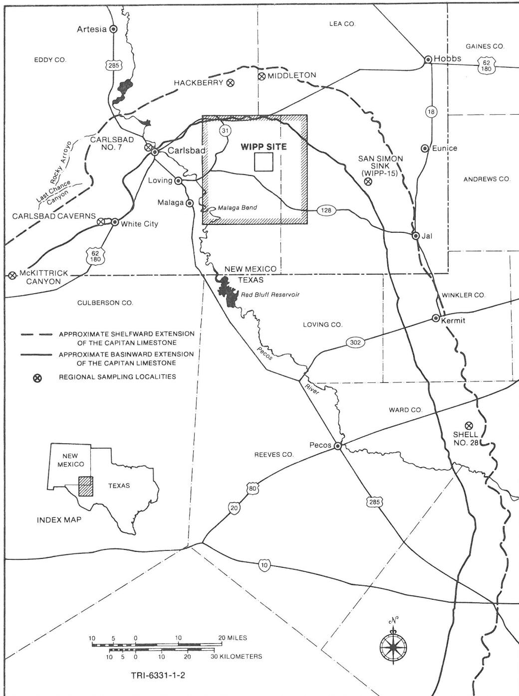
FIG. 1. Regional map of the Delaware Basin, southeastern New Mexico and West Texas. Approximate positions of basinward and shelfward extensions of the Capitan Limestone are taken from HISS (1975). Hachured rectangle is the area covered by Fig. 2.
