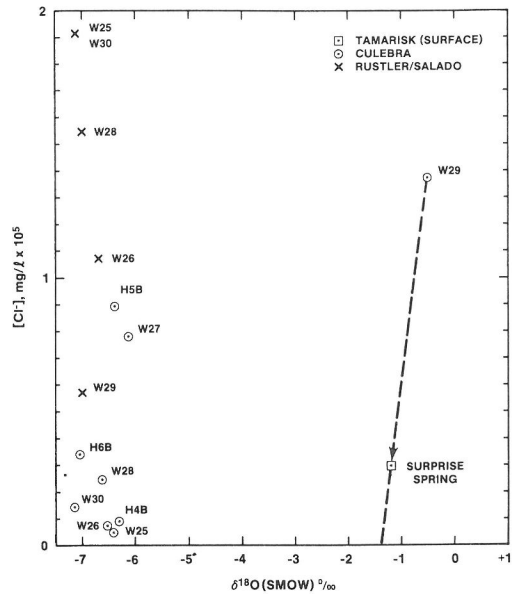
FIG. 10. Dissolved chloride versus \delta^{18}\text{O} for Rustler groundwaters in Nash Draw and at the WIPP site.
