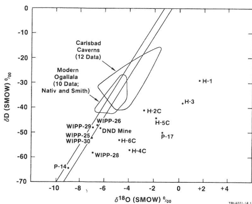
FIG. 7. Stable-isotope compositions of groundwaters from the Rustler/Salado contact.
